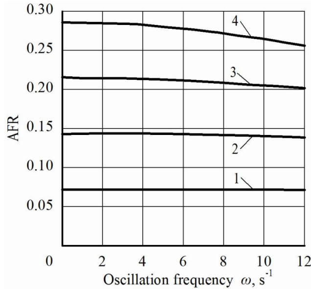
Fig. 1. Amplitude-frequency characteristics of the angular angle \varphi of the tractor when working out their disturbances in the form of fluctuations of the angle \beta of turning the reaper at different speeds of the unit: 1 – V_o = 1.0 \text{ m}\cdot\text{s}^{-1} ; 2 – V_o = 2.0 \text{ m}\cdot\text{s}^{-1} ; 3 – V_o = 3.0 \text{ m}\cdot\text{s}^{-1} ; 4 – V_o = 4.0 \text{ m}\cdot\text{s}^{-1} .
