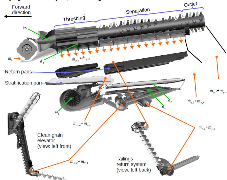
Fig. 1. Threshing, separation and cleaning system material flows.
